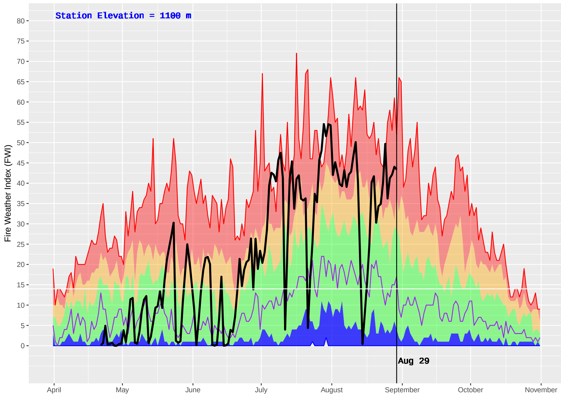
PALLISER (411) : Historical (1973–2016) and Current (2017) Noon Fire Weather Index (FWI)
