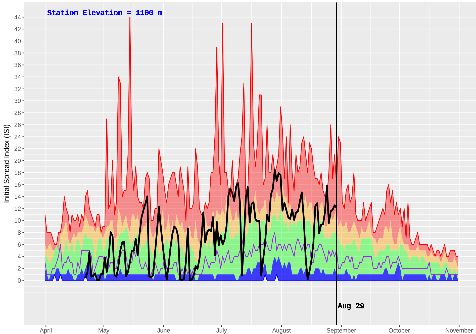
PALLISER (411) : Historical (1973–2016) and Current (2017) Noon Initial Spread Index (ISI)
