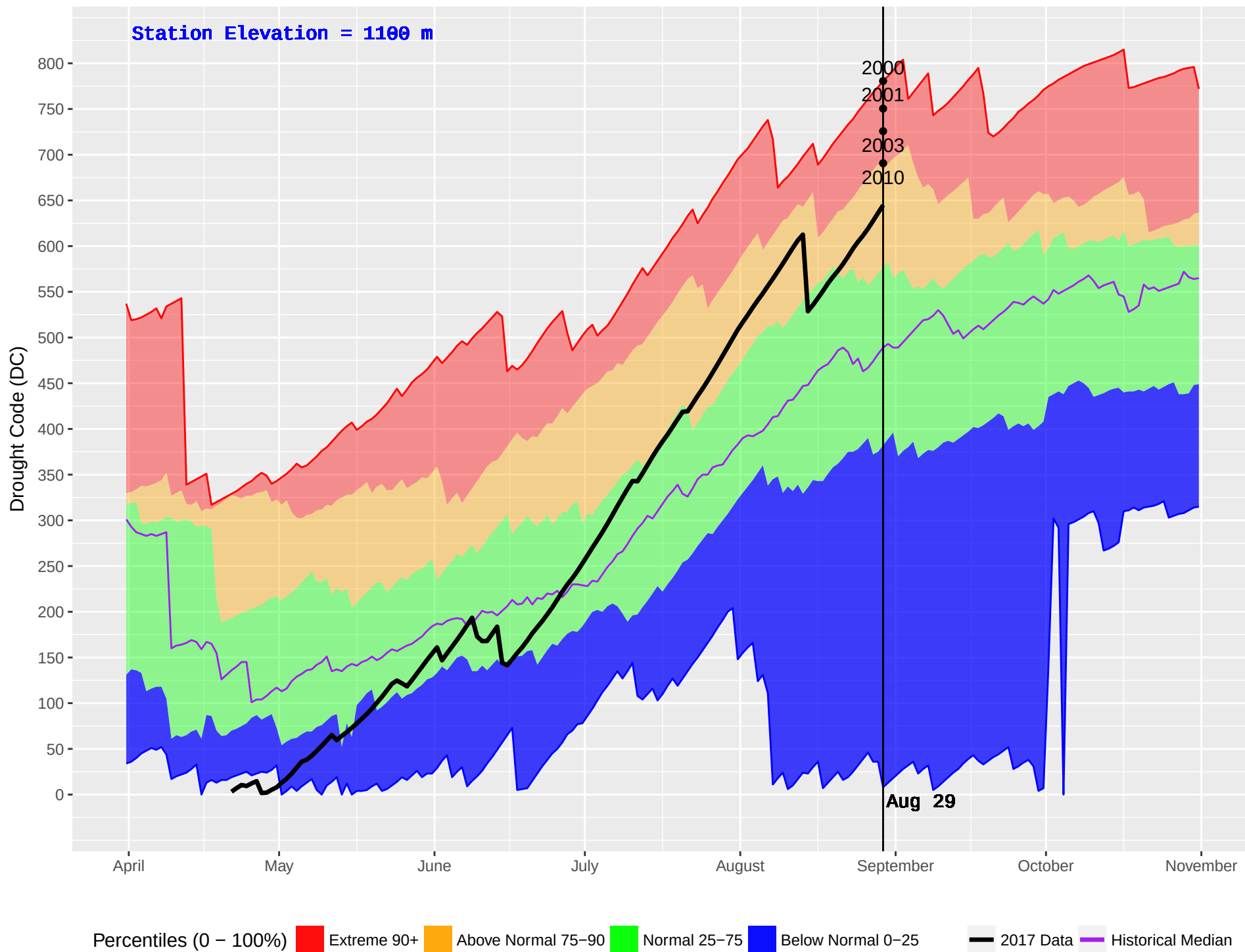
PALLISER (411) : Historical (1973–2016) and Current (2017) Noon Drought Code (DC)
